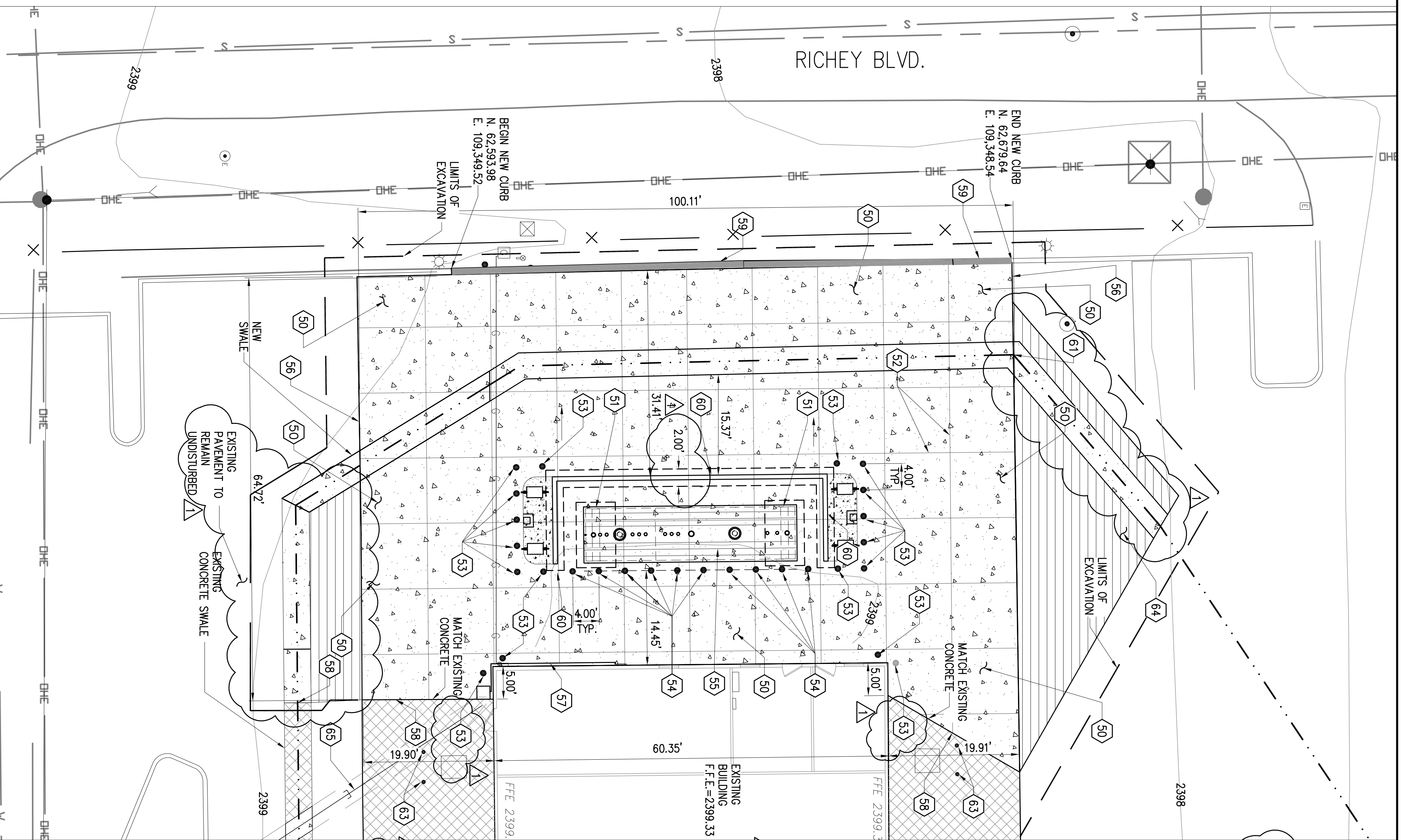
CIVIL SITE IMPROVEMENT PLAN SCALE: 1" = 10'
