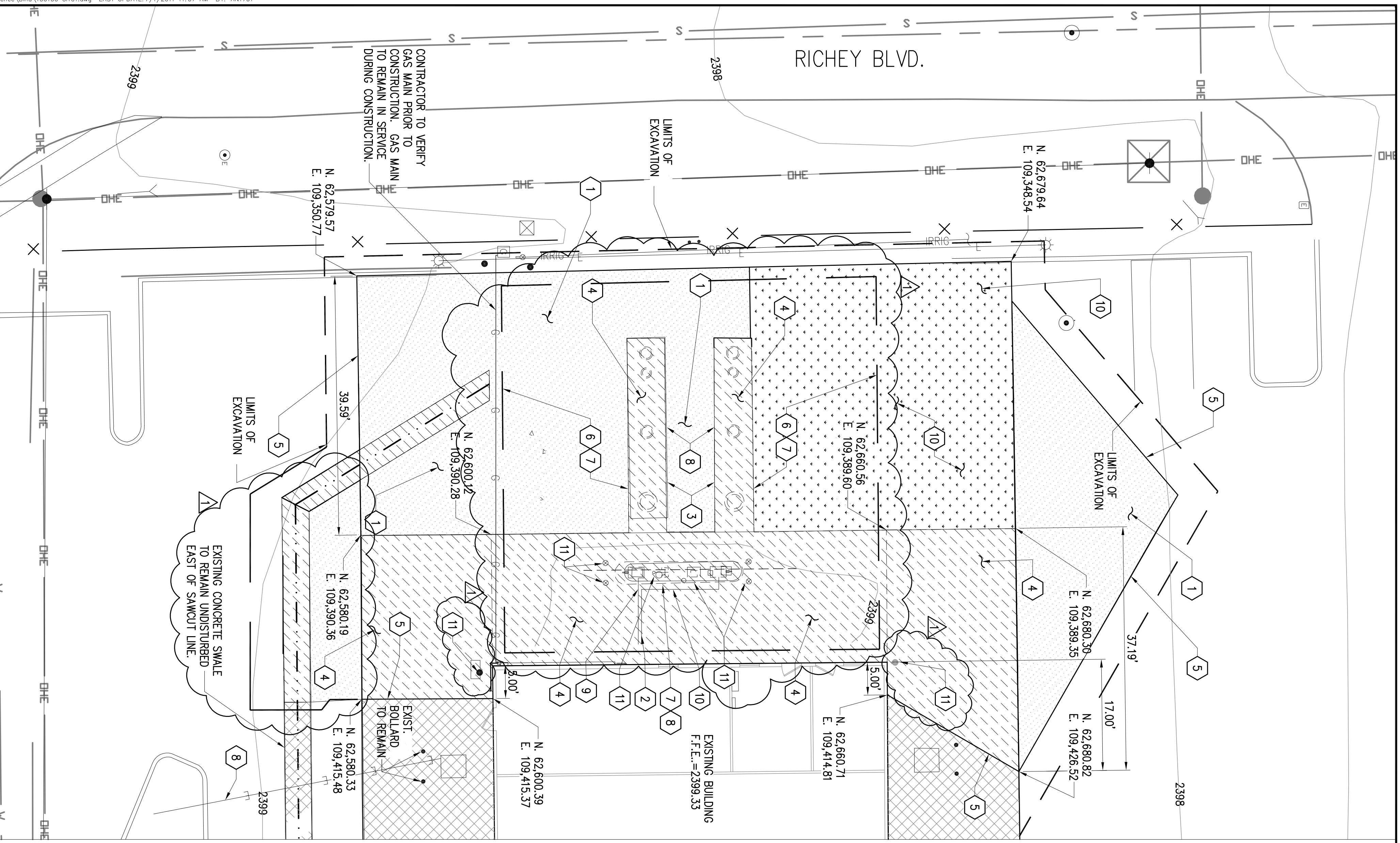
CIVIL DEMOLITION PLAN SCALE: 1" = 10'
